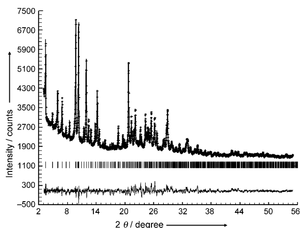
Figure 1. Observed (crosses) and calculated (lines) XRD patterns of as-synthesized DNL-1 as well as the difference profile (bottom). The short tick marks below the patterns give the positions of Bragg reflections.
